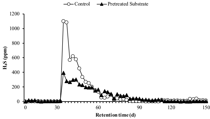
Figure 8: Daily variation in hydrogen sulphide (H 2 S) concentration during anaerobic digestion of untreated and biologically pretreated coconut coir lignocellulosic biomass
