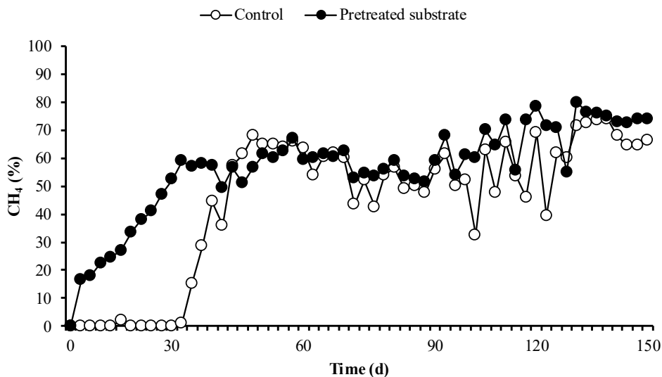
Figure 6: Daily variation in methane ( CH_4 ) content during anaerobic digestion of untreated and biologically pretreated coconut coir lignocellulosic biomass
