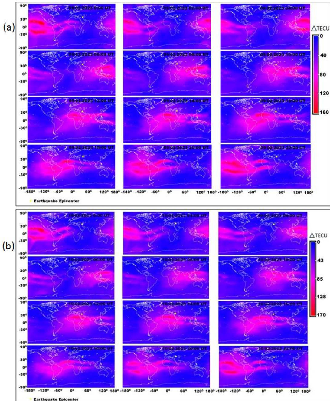
Figure 4: Spatial TEC maps above the epicenter of the M7.8 Turkey seismic event: (a) February 9 th , 2023, (b) February 10 th , 2023. The yellow star on Figures (4a) and (4b) indicate the epicentral position of the geo-quake; the legend indicates the TECU (TEC unit) within each Universal Time hour.
